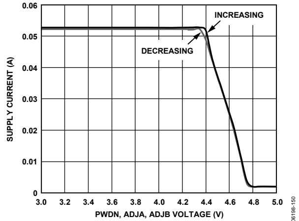
Figure 49. Supply Current vs. V_{PWDN} , V_{ADJA} , V_{ADJB}
